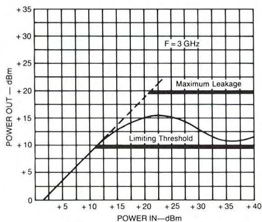
Fig. 2—Model 726 power in vs. power out
