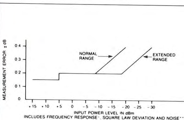
Fig. 1A-Model 478A/N436A accuracy
