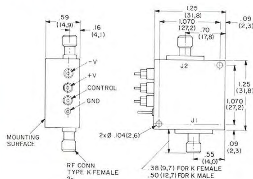
MODEL D1959 Wt: 1 oz. (28 gm) approx.
