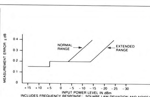
Fig. 1B-Model 490/M439, 490/MK439, 490/A439 accuracy
