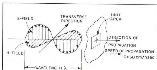
Fig. 2-E- and H-Field Relationships of an Electromagnetic Wave in Free Space
