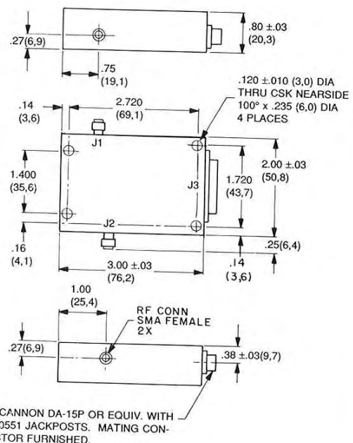
MODEL 3458H Wt: 4 oz. (113 gm) approx.
