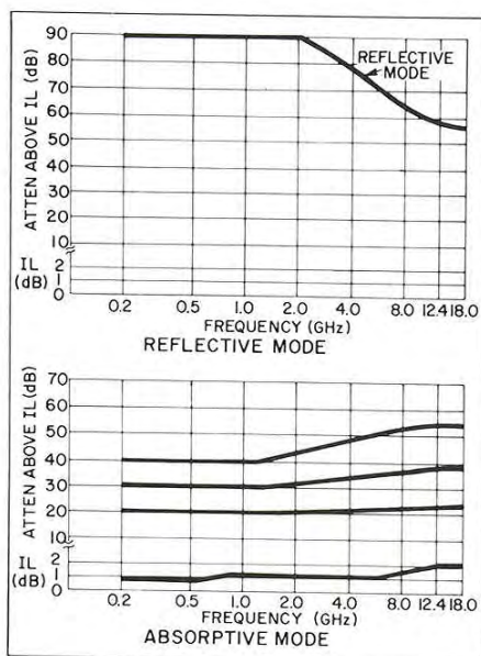
Fig. 3-Typical response curves of Model M186C
