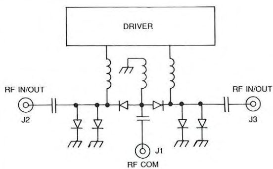
Fig. 1—Series F90 SPDT schematic diagram
