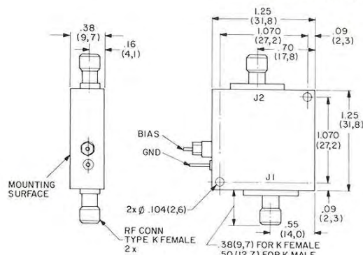
MODEL 1959 Wt: .8 oz. (23 gm) approx.
