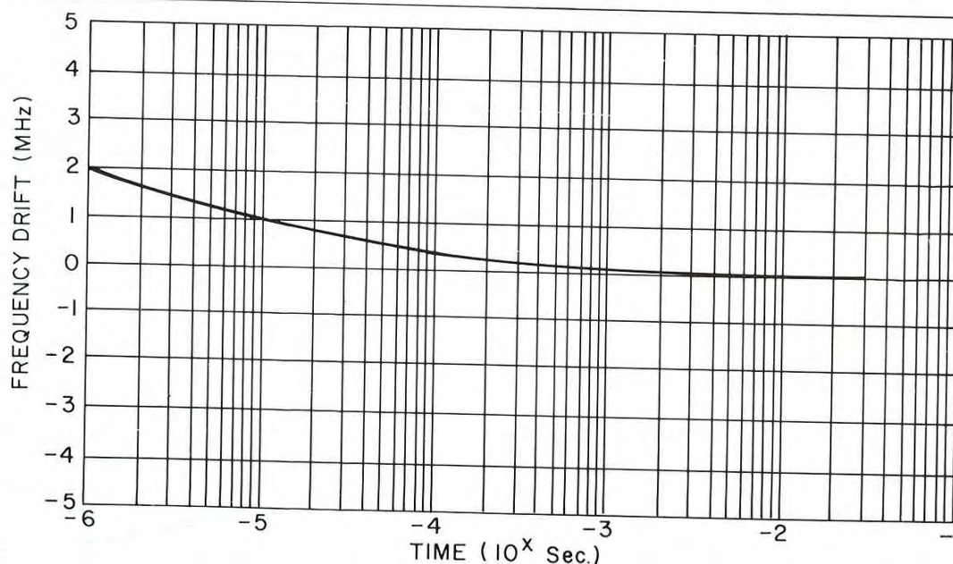
Fig. 6-Measured settling time of 8-12 GHz VCO
