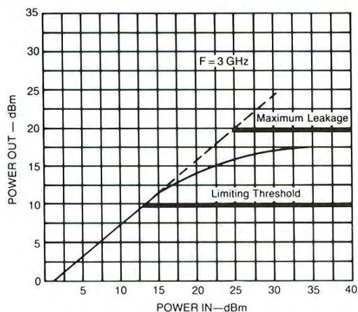
Fig. 1—Model 725 power in vs. power out
