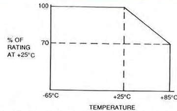
Fig. 6-Models M186C, LM186C, M189C, LM189C, M190C and LM190C, survival power derating factor
