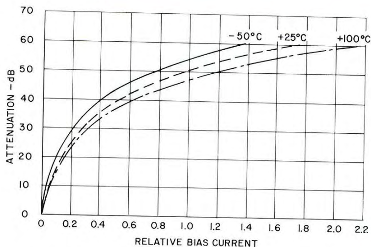
Fig. 3-Series 195, typical effects of temperature on attenuation
