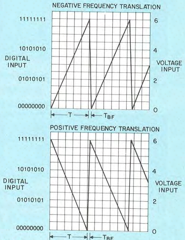
Fig. 3-Series 77 and Series 78 input requirements
