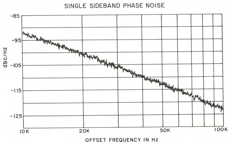
Fig. 7-Measured phase noise of 12 GHz DRO
