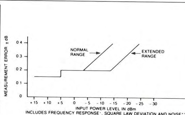
Fig. 1B-Model 478A/M438A, MK438A accuracy
