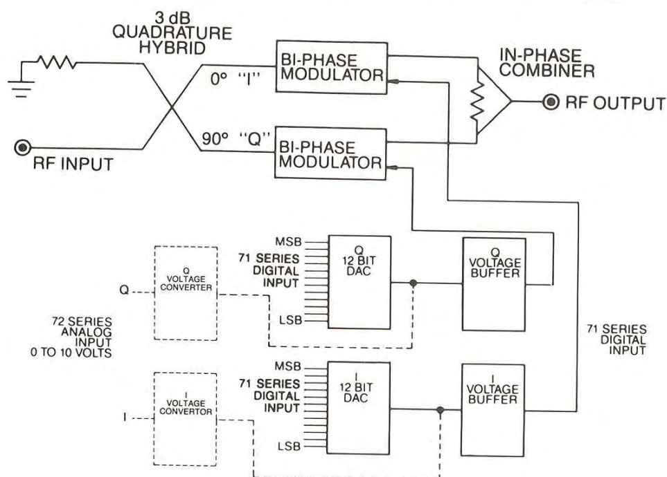
Fig. 1-Series 71, 72 Block Diagram
