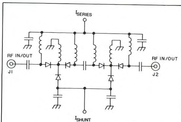
Fig. 1-Series D196, rf schematic diagram
