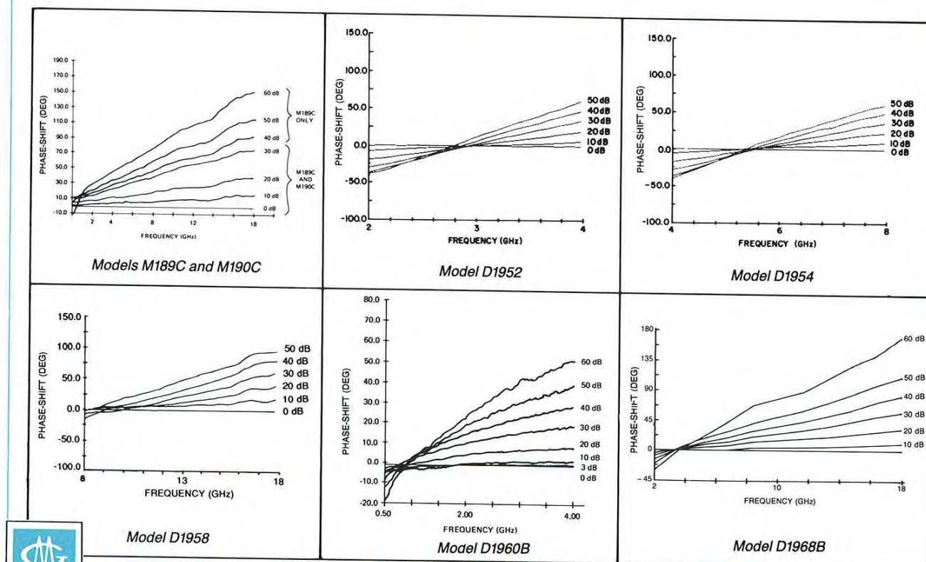
Fig. 6 Typical Phase vs. Attenuation
