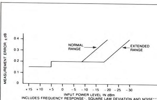
Fig. 1A-Model 490/N439 accuracy
