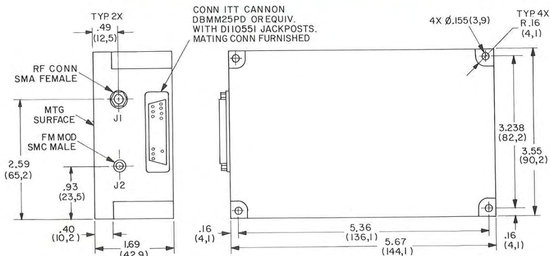
MODELS D6020, D6026, D6040, D6080 AND D6120 DTOs Wt: 23.1 oz. (655 gm) approx.
