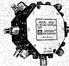
9160-500 (DRIVERLESS)
