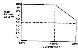
Fig. 1B. — DM86 units
