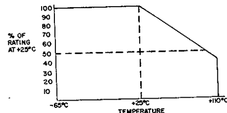
Fig. 4-Models D1960A and D1962A, survival power derating factors
