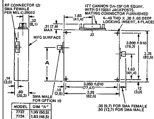
MODELS 7722 AND 7724 Wt: 6 oz. (170 gm) approx.
