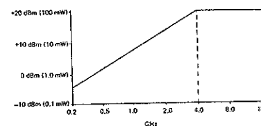
Fig. 4-Model 3250, survival power derating factors.
