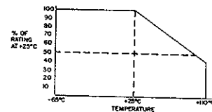
Fig. 1B. — F91/F92 units
