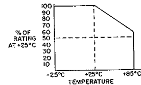
Fig. 2-Series 329, survival power derating factors
