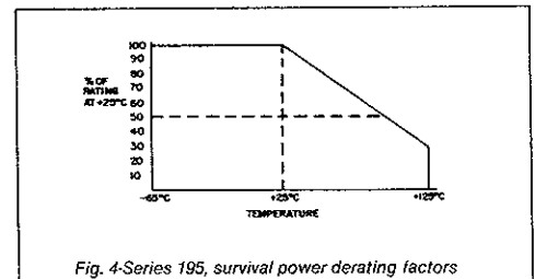
Fig. 4-Series 195, survival power derating factors
