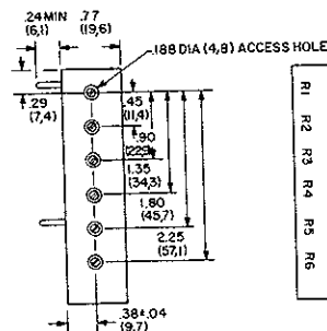
MODEL 311 DRIVER Wt: 4 oz. (113 gm) approx.
