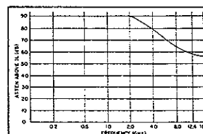
Fig. 3-Typical DM186CH-31 response curve
