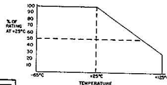
Fig. 1A. — M86 units
