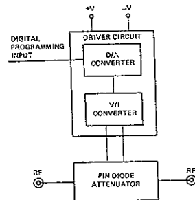
Fig. 1-Model 3250, block diagram
