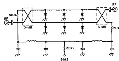
Fig. 1-Models 1951-1958, rf schematic diagram
