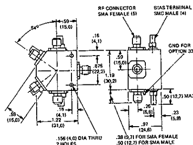
MODEL M871A Wt: 2.5 oz. (70 gm) approx.
