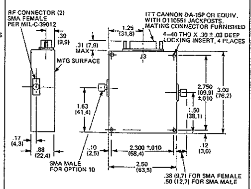
MODEL 7728 Wt: 4 oz. (113 gm) approx.
