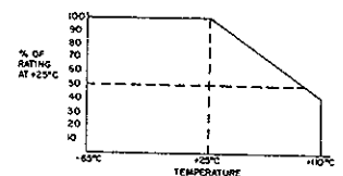
Fig. 1C. — FM86 units
