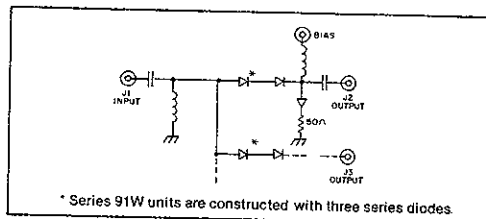
Series 91T, 92T and 91W schematic diagram
