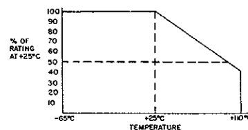
Fig. 3-Models 3460 and 3462, survival power derating factors
