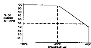
Fig. 1A — Units with integrated drivers
