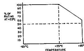
Fig. 1 — Survival power derating factors
