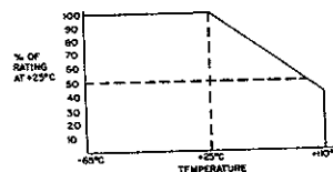
Fig. 1A — Integrated units
