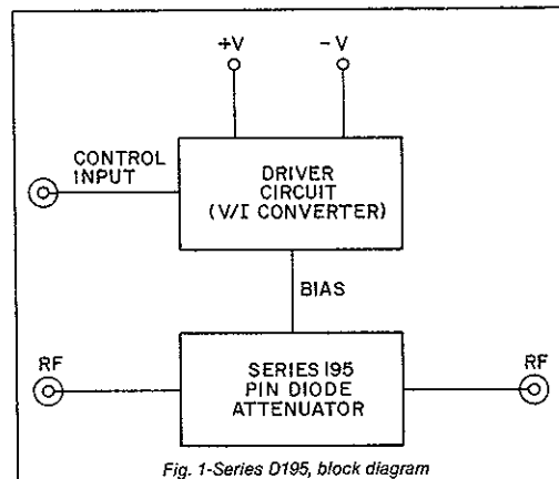
Fig. 1-Series D195, block diagram
