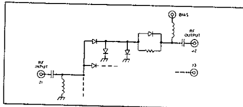
Model 9120HT-500 schematic diagram
