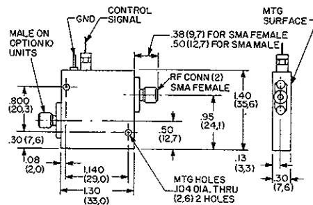
MODELS 1954, 1955 AND 1956 Wt: 1 oz. (28 gm) approx.
