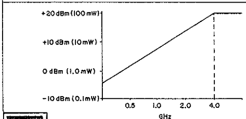
Fig. 2-Model 3460, maximum peak and average operating power without performance degradation
