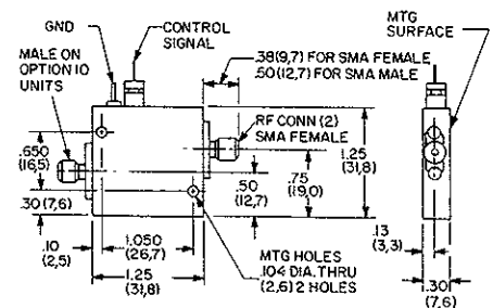
MODEL 1958 Wt: 1 oz. (28 gm) approx.
