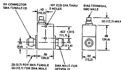
SERIES M86 SWITCHES Wt: 1 oz. (28 gm) approx.
